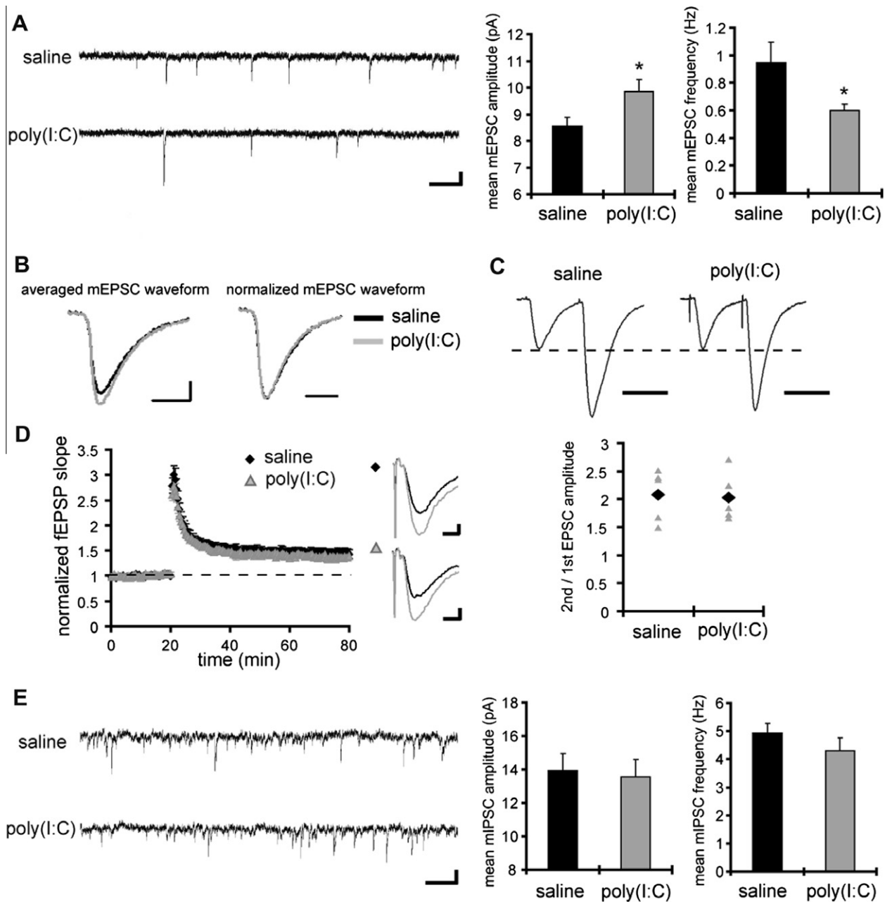
Fig. 1. CA1 pyramidal neurons in MIA offspring display a reduced frequency and an increased amplitude of mEPSCs, but no significant difference in mIPSCs. (A) Typical recordings and quantification of mEPSCs from CA1 pyramidal neurons are shown (saline: n = 11 neurons, poly(I:C): n = 12 neurons, 4 pairs of animals) (scale bar = 500 ms, 10 pA) ( p < 0.05 relative to control). (B) Averaged mEPSC waveforms from animals used for the analysis in A are shown on the left. The mEPSC waveform in MIA offspring shows larger amplitude compared to that in control animals. To examine the kinetics of the waveforms, the amplitudes of mEPSC waveforms are normalized on the right. There is no significant difference in kinetics of mEPSCs between the groups. (C) Whole-cell voltage-clamp recordings were performed in CA1 pyramidal neurons under inhibitory blockade with the GABA receptor antagonists bicuculline (10 \mu M) and CGP55845 (1 \mu M). Membrane potential was clamped at -60 mV. Paired-pulse facilitation (PPF) was analyzed at Schaffer–collateral–CA1 synapses. The top panel shows representative waveforms (interstimulus interval is 50 ms; scale bar = 50 ms), and the bottom panel shows the PPF ratio (2nd/1st EPSC amplitude) of individual recordings (gray triangles), and the mean values (black diamonds) ( n = 5 neurons for each group, 3 pairs of animals). (D) Extracellular field recordings were performed at Schaffer–collateral–CA1 synapses under fast inhibitory transmission block with the GABA A receptor antagonist bicuculline. The left panel shows the normalized fEPSP slope from control animals (black diamonds) and MIA offspring (gray triangles) and LTP was induced at 20 min by a single train of 100 stimuli at 100 Hz. The right panel shows representative waveforms before (black) and after (gray) LTP induction (scale bar = 0.2 mV, 5 ms). No significant difference is observed in LTP magnitude between animal groups ( n = 8 slices for each group, 3 pairs of animals). (E) Typical recordings and quantification of mIPSCs from CA1 pyramidal neurons are shown ( n = 12 neurons for each group, 3 pairs of animals). A cesium chloride-based solution was used as the internal solution of patch pipettes and recordings were made at 28 °C in the presence of TTX (1 \mu M), NBQX (20 \mu M) and APV (50 \mu M) to block excitatory synaptic transmission. The extracellular potassium concentration was increased from 2.5 to 5 mM to enhance the frequency of miniature synaptic events. No significant difference is observed in mIPSC amplitude or frequency between the groups.
