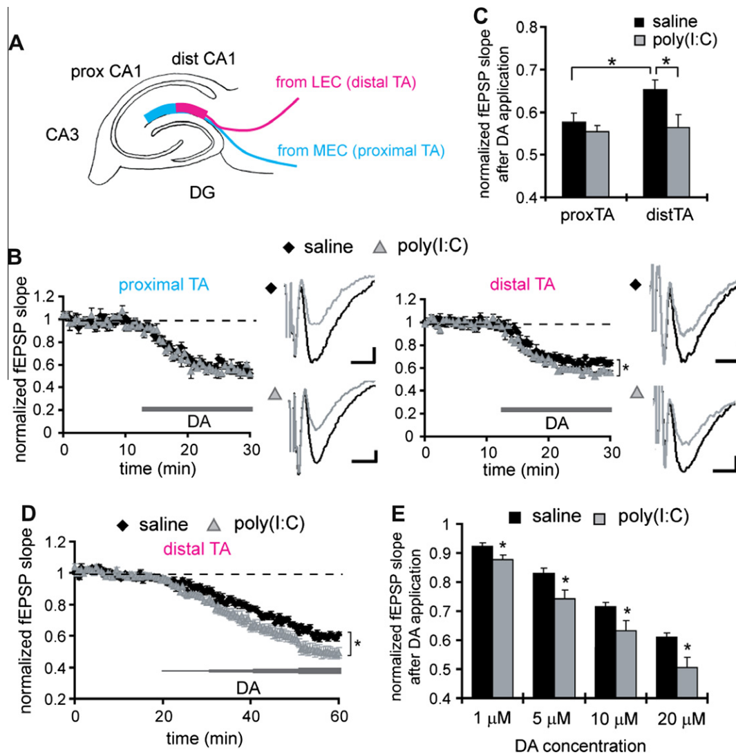
Fig. 2. The offspring of poly(I:C)-treated mothers display increased DA-induced depression at distal temporoammonic-CA1 synapses. (A) A schematic diagram is shown depicting the two distinct axonal projections in the TA pathway from MEC and LEC. (B) Extracellular field recordings are obtained simultaneously from proximal and distal TA-CA1 synapses. For each recording from proximal or distal TA-CA1 synapses, the left panels show the normalized fEPSP slopes from control (black diamonds) and MIA offspring (gray triangles), and the right panels show representative traces of fEPSP waveforms before (black) and after (gray) DA application (scale bar = 0.05 mV, 5 ms). The test pulse was applied every 30 s and DA (20 μM) was bath applied during the time indicated by the thick line ( *p < 0.05 relative to control) (saline: n = 7 slices, poly(I:C): n = 6 slices, 4 pairs of animals). (C) In hippocampal slices prepared from control animals, DA induces a significantly larger depression at proximal compared to distal TA-CA1 synapses. While the slices prepared from MIA offspring show a normal DA-induced depression at proximal synapses, they exhibit a significantly larger depression at distal TA-CA1 synapses, compared to controls ( *p < 0.05 ). (D) Hippocampal slices prepared from MIA offspring show increased DA-induced depression at distal TA-CA1 synapses. The DA concentration was increased every 10 min, from 1 to 20 μM ( *p < 0.05 relative to control). (E) Analysis of the data in D is shown. The mean fEPSP slopes at 5–10 min after the application of each designated concentration of DA were analyzed. Slices prepared from MIA offspring show a significantly larger depression at each DA concentration examined ( n = 12 slices for each group, 8 pairs of animals) ( *p < 0.05 relative to control).
