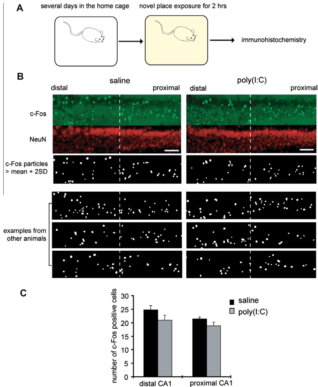
Fig. 4. The offspring of poly(I:C)-treated mothers display comparable c-Fos expression in area CA1 pyramidal neurons following novel place exposure. (A) A schematic diagram of the behavioral procedure is shown. After mice were accommodated to the new home cage for a few days, they were moved to a novel cage. After a 2 h exposure, immunohistochemistry on the hippocampus was carried out. (B) Examples of c-Fos expression in the pyramidal layer of area CA1 are shown. The pyramidal layer was divided into equal proximal and distal regions. The c-Fos signals that are larger than the mean + two times the standard deviation, were quantified using ImageJ (see Section 2 for details) (scale bar = 100 μm). (C) The number of c-Fos signals was quantified in proximal and distal regions of CA1 pyramidal layer ( n = 5 pairs of animals, 2 sections analyzed from each).
