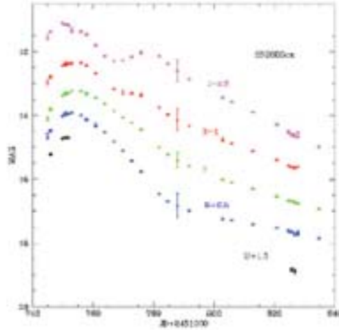
SN2000cx is a Type Ia Supernova in the outer part of NGC 524 at about 35 Mpc distance, below and to the right of the brightest star in the figure on the right. Gamma ray observations can determine how much of the light from the supernova (light curves shown) is powered by radioactive decays from isotopes that are formed in the event.
