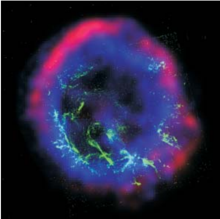
Color composite of the supernova remnant E0102-72: X-ray (blue), optical (green), and radio (red). E0102-72 is the remnant of a star that exploded in a nearby galaxy known as the Small Magellanic Cloud. The Chandra X-ray Observatory image, shown in blue, shows gas that has been heated to millions of degrees Celsius by the rebounding, or reverse shock wave. The X-ray data show that this gas is rich in oxygen and neon. These elements were created by nuclear reactions inside the star and hurled into space by the supernova.
