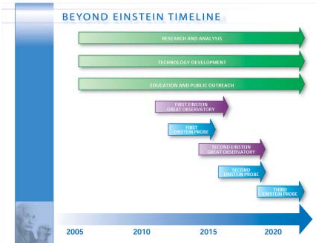
constellation-x
