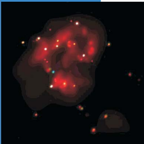
Chandra X-ray Observatory image of possible intermediate mass black holes accreting gas in the Antennae pair of colliding galaxies.
