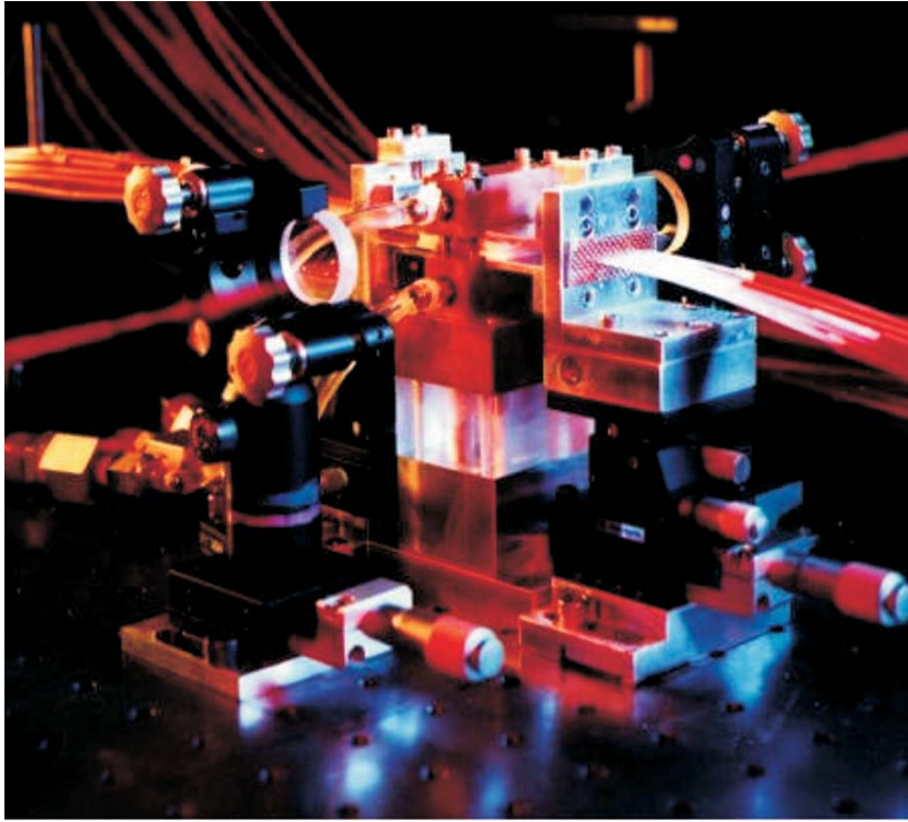
The Big Bang Observer will require powerful space-qualified lasers. Here a 125 W laser (scalable to 30 kW) is shown under test.
