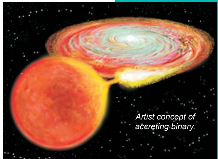
supernovae
