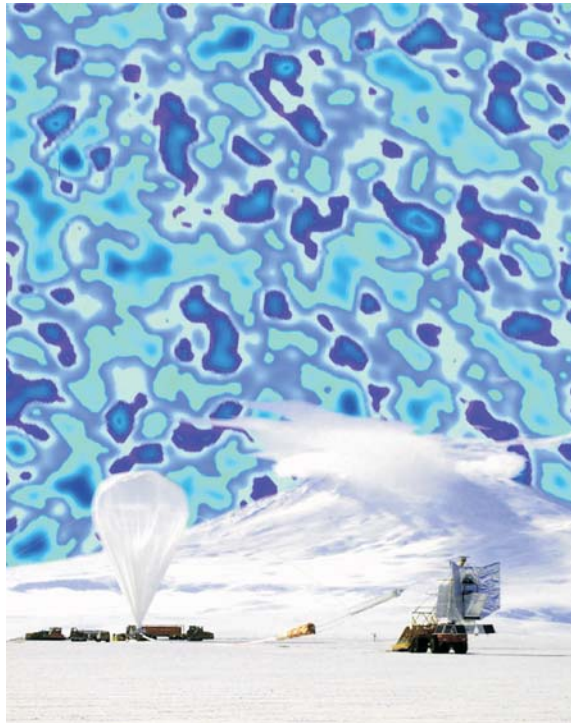
The BOOMERANG measurements performed under the supporting research and analysis program provided key measurements on the shape of the Universe from observations of the cosmic microwave background.
