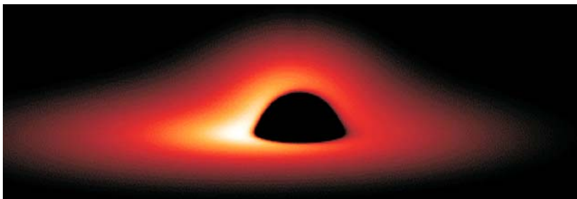
A simulated Black Hole Imager view of an accretion disk around a black hole. The bending of light rays by the black hole makes the back side of the disk appear raised.
