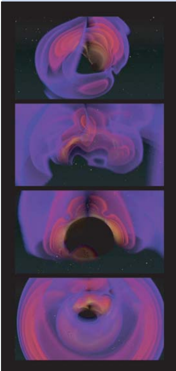
Supercomputer calculation of the gravitational waves produced in the merger of two supermassive black holes (AEI-ZIB)
