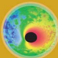
black holes
